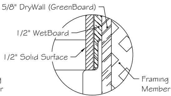
Finish Out Of Detail "A" (For Solid Surface Applications)
