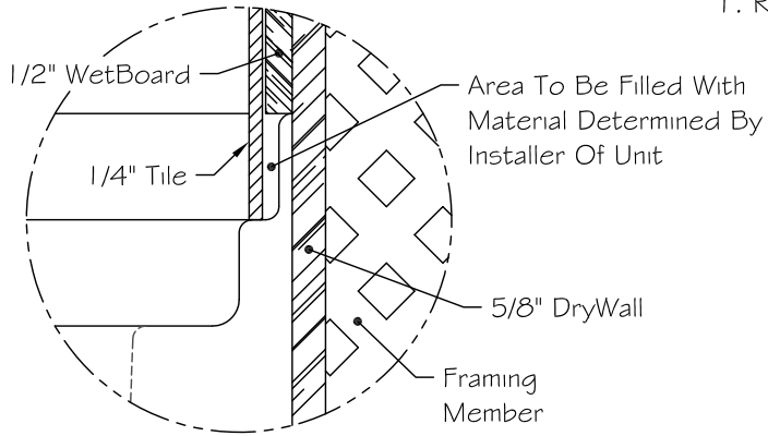
Finish Out Of Detail "A"
